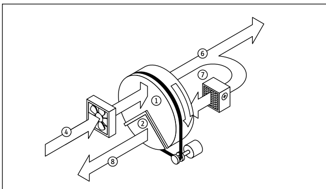
Fig.: Functional principle
