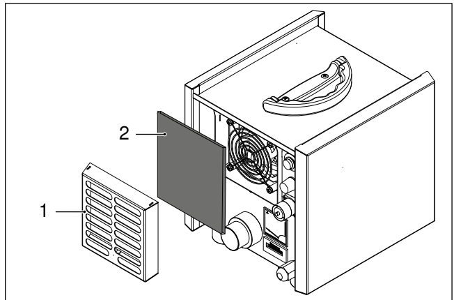
Fig.: Air filter replacement TTR 200/300
