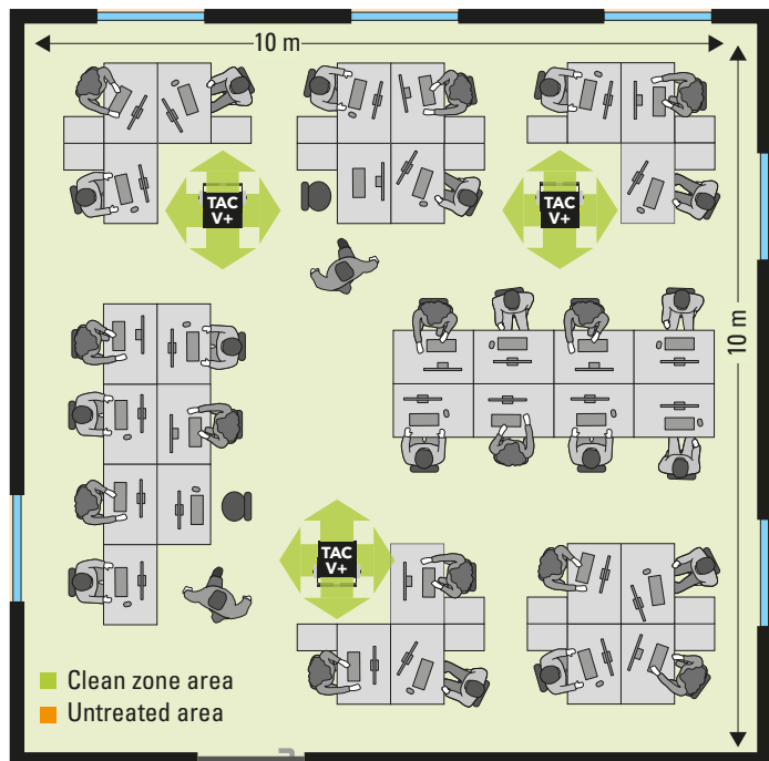
Example call center: With an area of 10 x 10 m at a room height of 2.5 m, the office zone shown has an air volume of 250 m 3 , which 3 TAC V+ can circulate 19 times per hour (air capacity 4,800 m 3 /h), which corresponds to an air exchange rate (LW/h) of 19.
